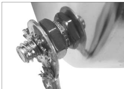
Step 15 - Slide Ring Terminal Wire Assembly onto Stud & Lock Washer over Ring
